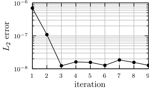
Figure 6: L_2 error for the d = 5 example.
