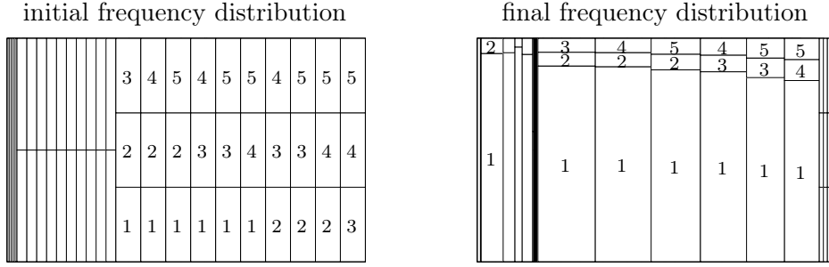
Figure 7: Depiction of the frequency distribution in iteration 1 and 9 in the ANOVA terms for the d = 5 example.
