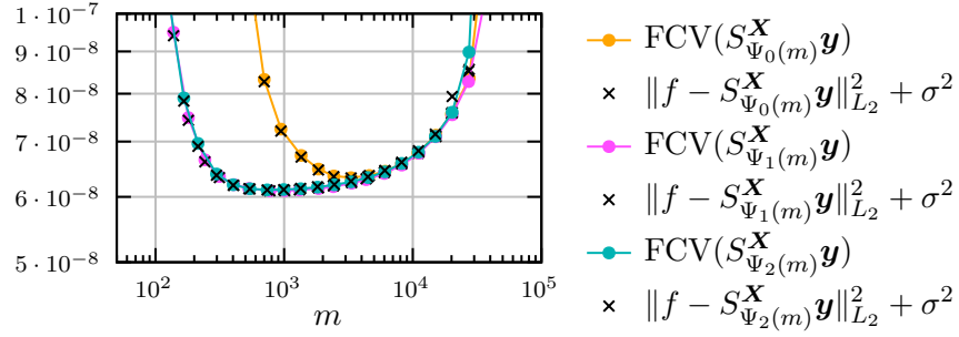
Figure 5: Cross validation and L_2 error for the d = 2 example with Gaussian noise.
