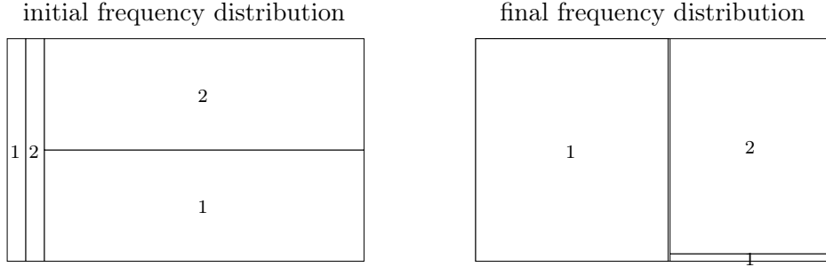
Figure 4: Depiction of the frequency distribution in iteration 1 and 9 in the ANOVA terms for the d = 2 example.
