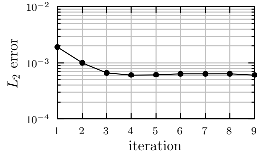
Figure 9: L_2 error for the d = 10 example.
