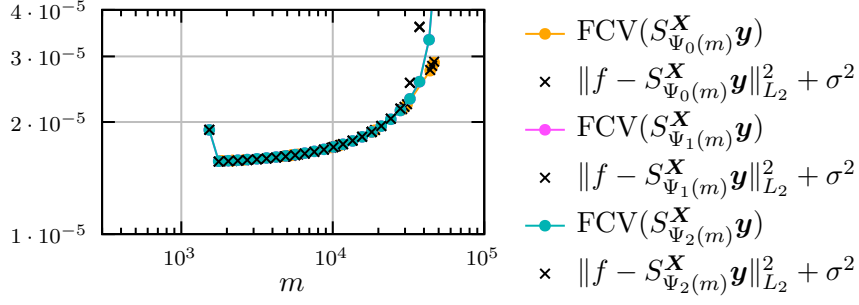
Figure 8: Cross validation and L_2 error for the d = 5 example with Gaussian noise.
