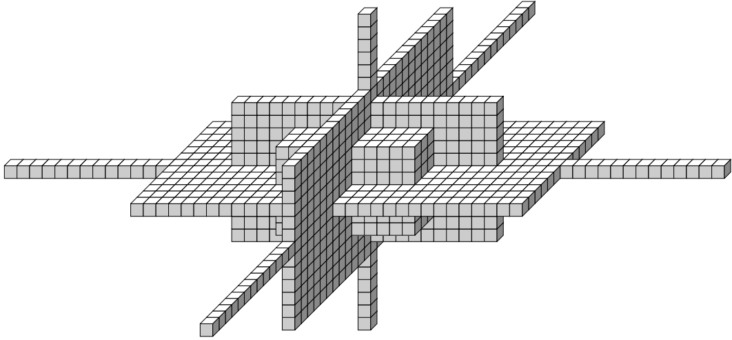
Figure 1: Example frequencies in dimension d = 3 used in ANOVA approximation with 12 bandwidth parameters.
