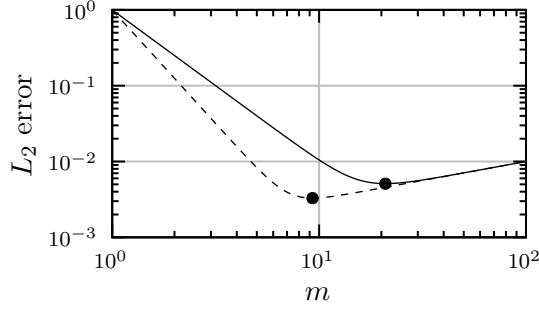
Figure 2: Error behavior \|S_{\Psi(m)}^{\mathbf{X}} \mathbf{y} - f\|_{L_2}^2 \lesssim m^{-2s_\Psi} + \sigma^2 m/n for s_\Psi = 2 (solid) and s_\Psi = 3 (dashed) in the presence of noise.
