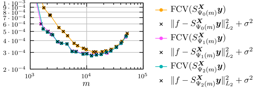
Figure 11: Cross validation and L_2 error for the d = 10 example with Gaussian noise.
