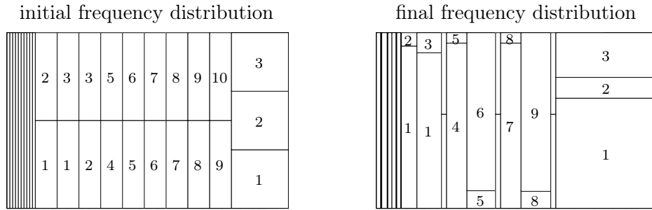
Figure 10: Depiction of the frequency distribution in iteration 1 and 9 in the ANOVA terms for the d = 10 example.
