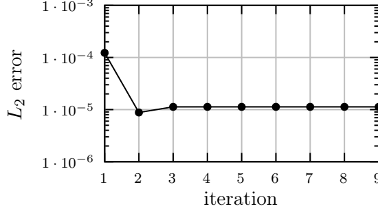
Figure 3: L_2 error for the d = 2 example.
